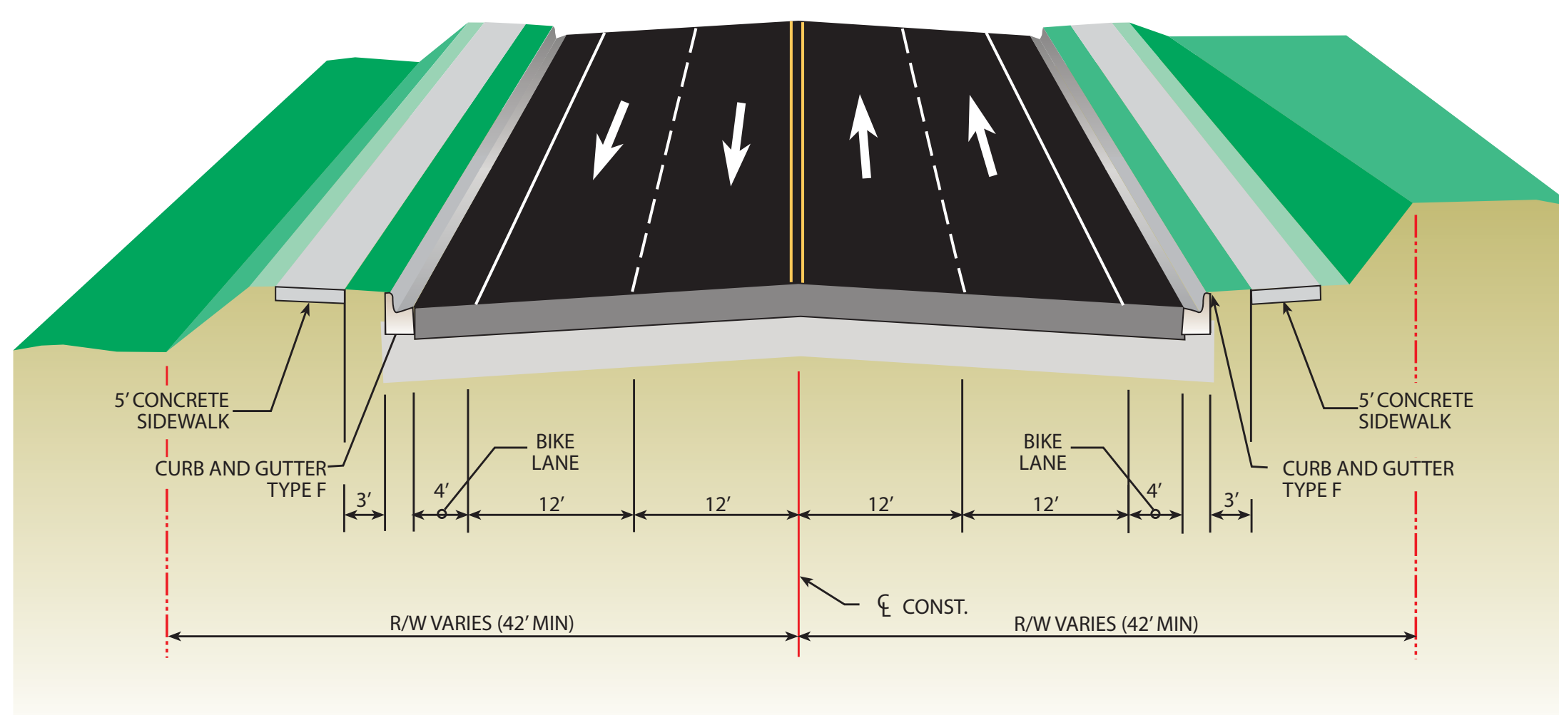
TYPICAL SECTION #3 Urban Section (4-Lane Undivided) Design (Maximum) Speed = 40 MPH
