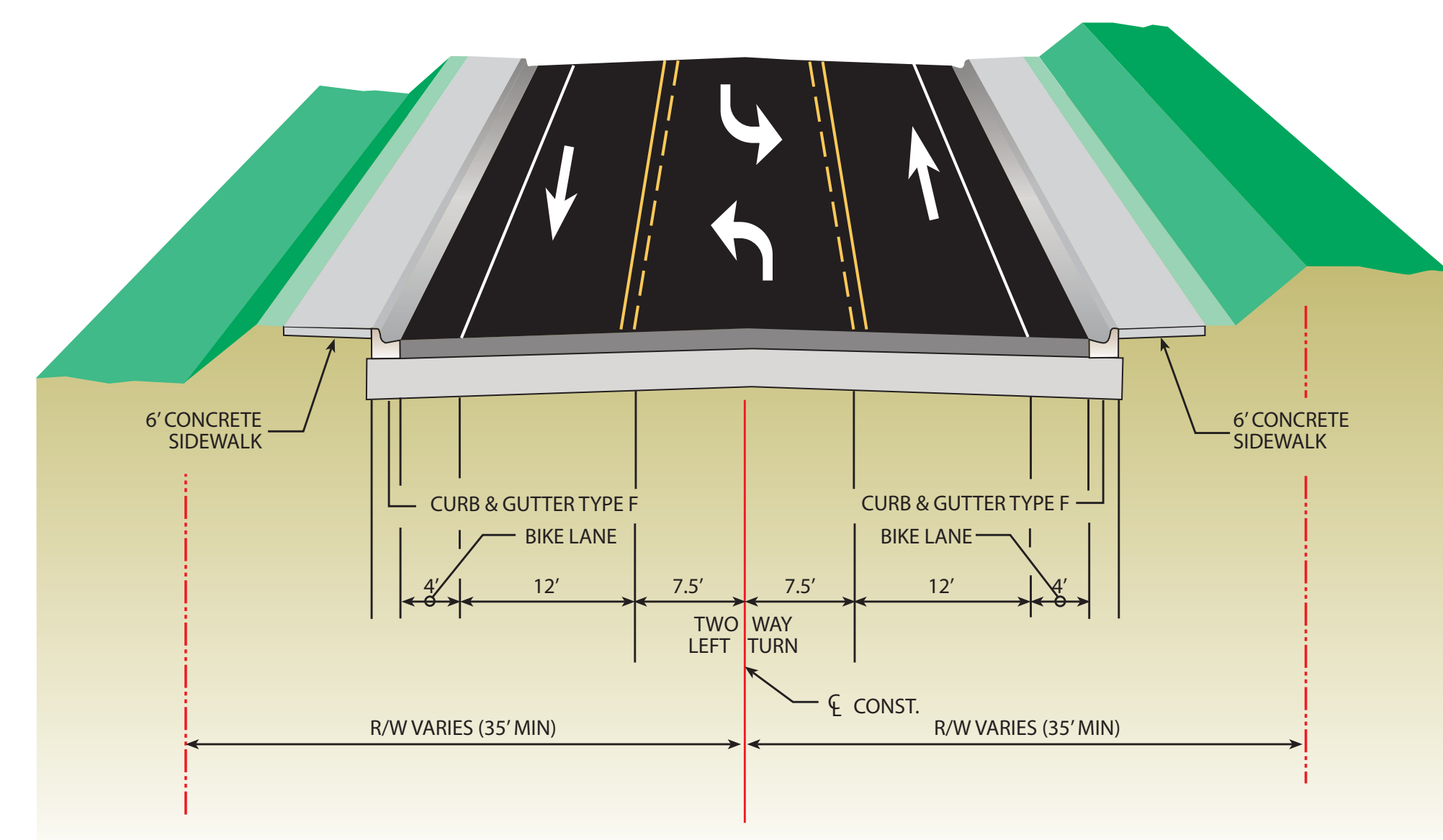
TYPICAL SECTION #6 Urban Section (3-Lane Undivided) Design (Maximum) Speed = 40 MPH
