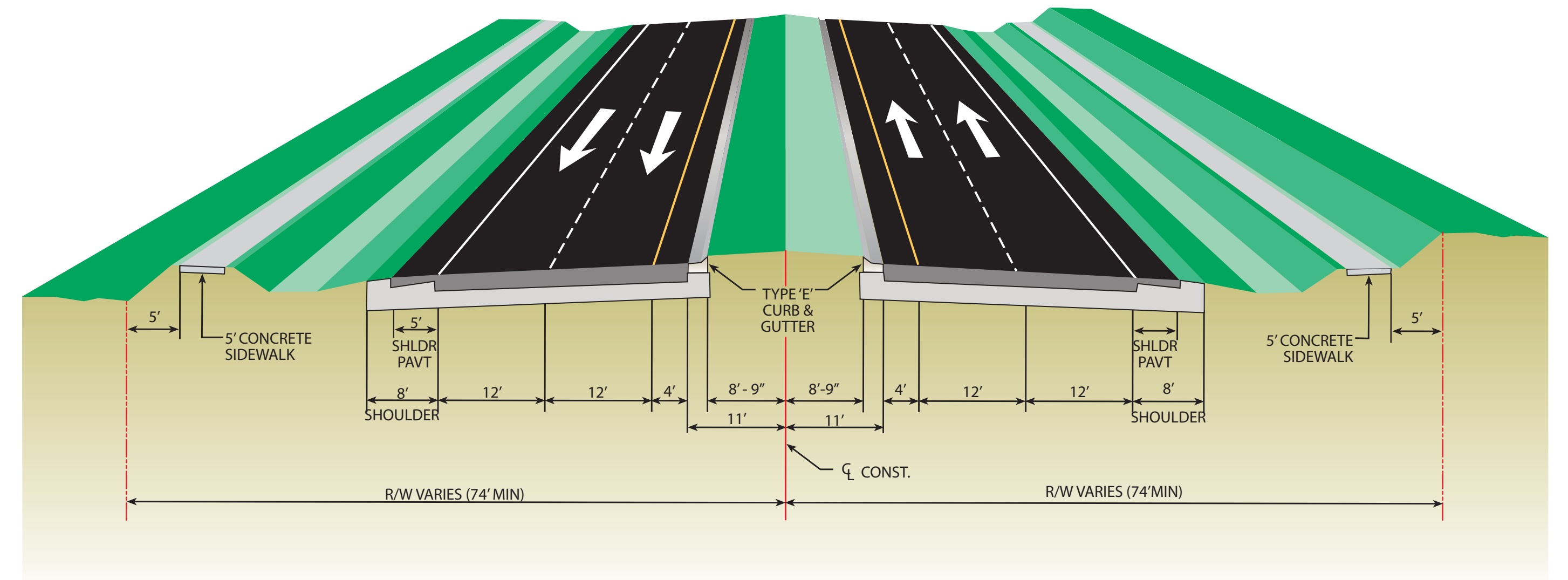
TYPICAL SECTION #2 High Speed Urban / Sub-Typical Section with Curb Inside and Flush Outside Design (Maximum) Speed = 50 MPH
