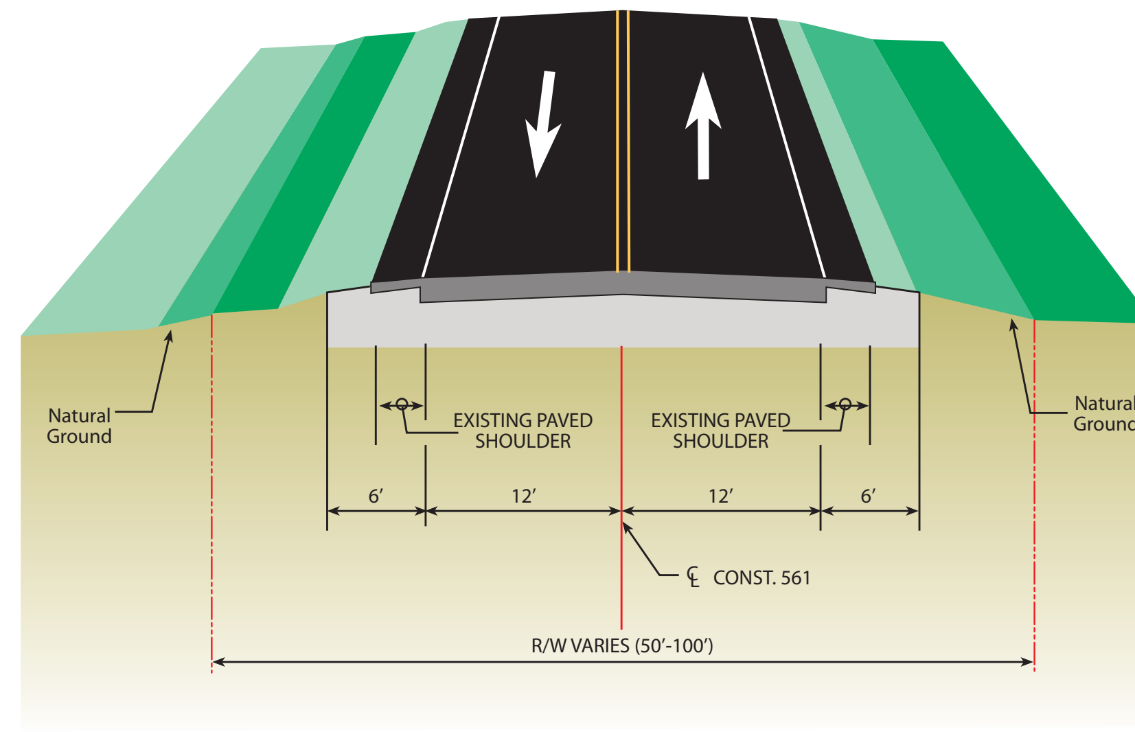
Existing Typical Section Posted Speed = 40 / 50 MPH
