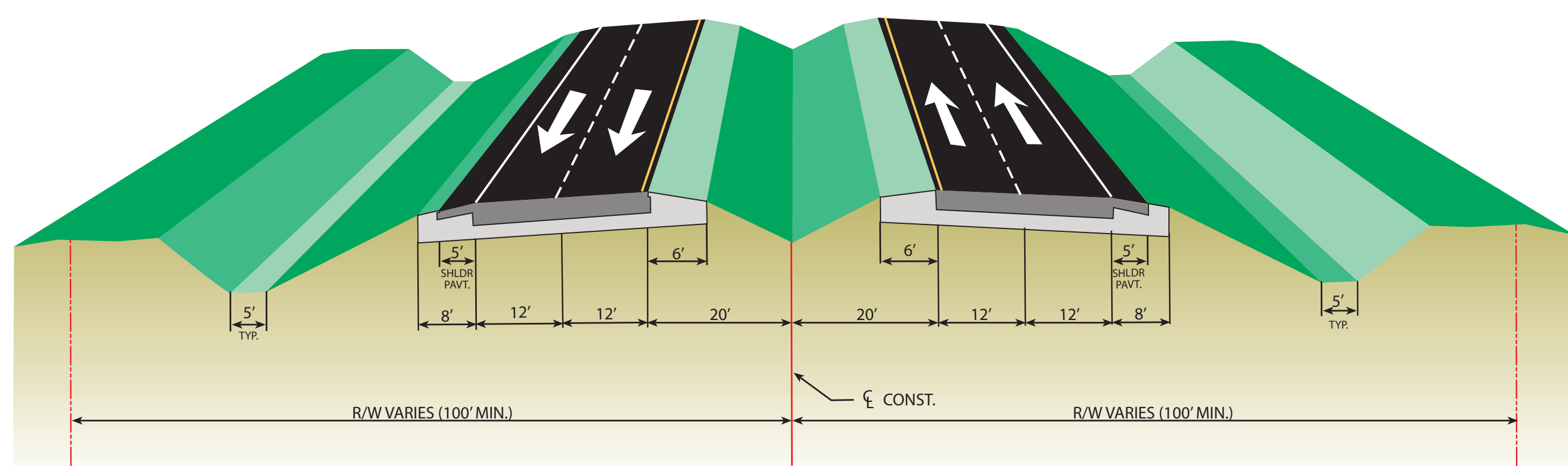
TYPICAL SECTION #1 Rural Section Design (Maximum) Speed = 50 MPH
