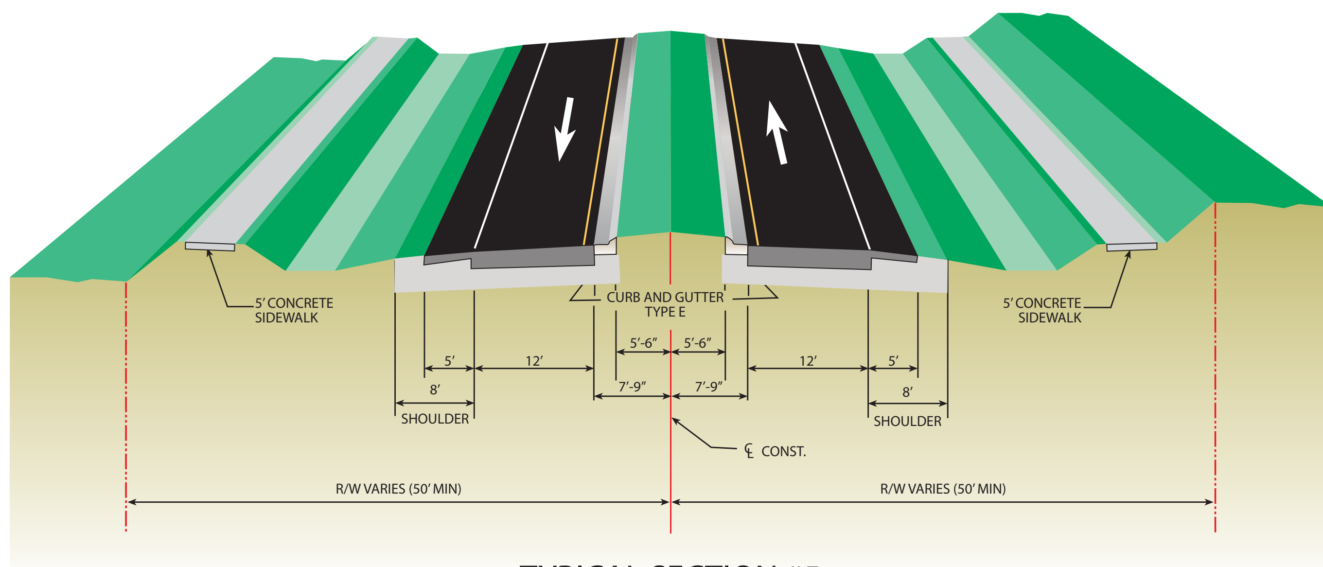
TYPICAL SECTION #5 Urban Section (2-Lane Divided) (Future 4-Lane) Design (Maximum) Speed = 40 MPH
