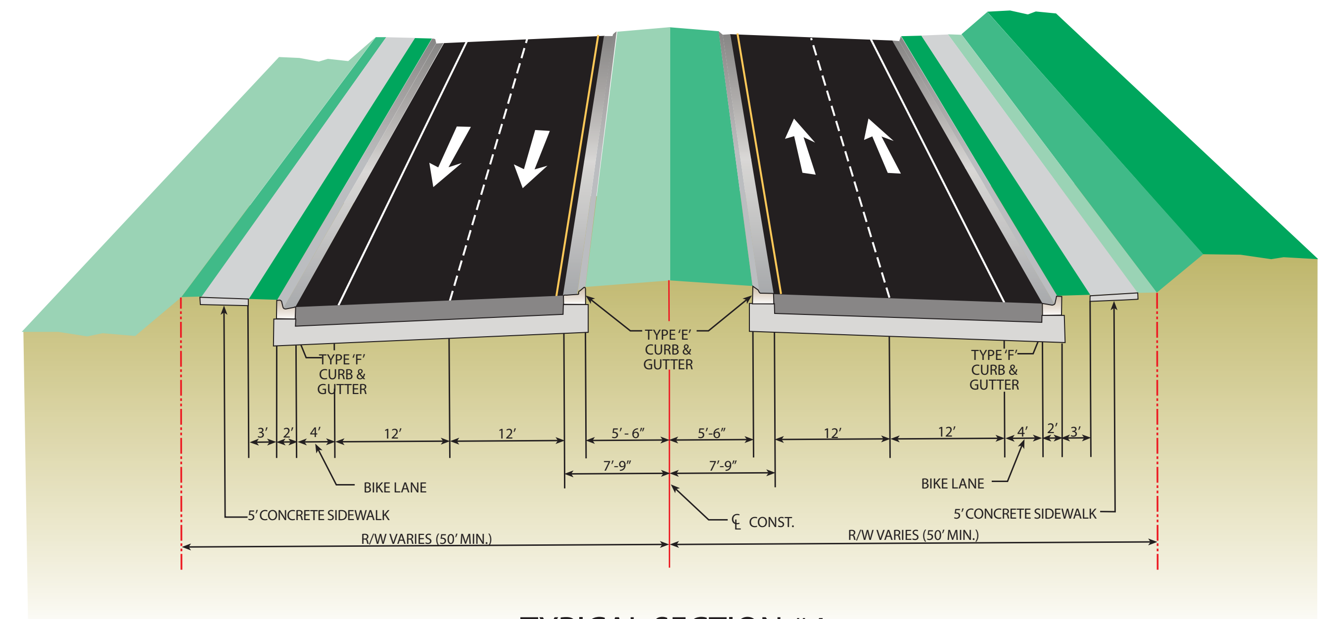
TYPICAL SECTION #4 Urban Section (4-Lane Divided) Design (Maximum) Speed = 40 MPH
